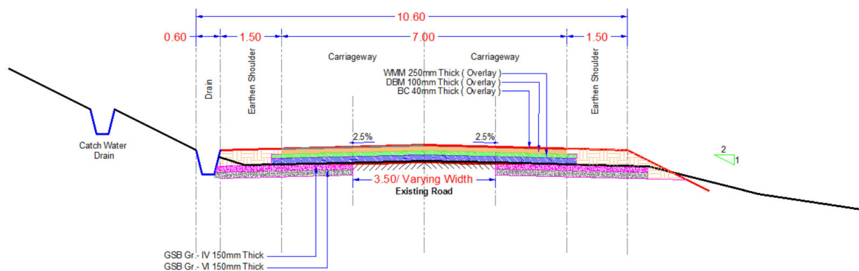
Figure B5: Typical Cross-section 3A
