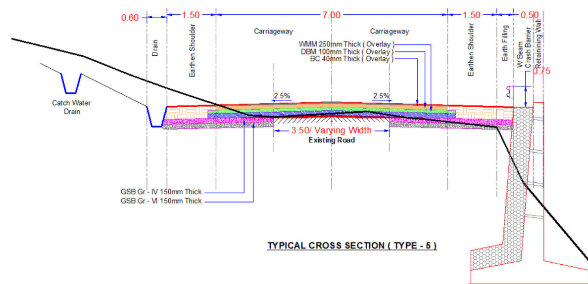
Figure B7: Typical Cross-section 5
