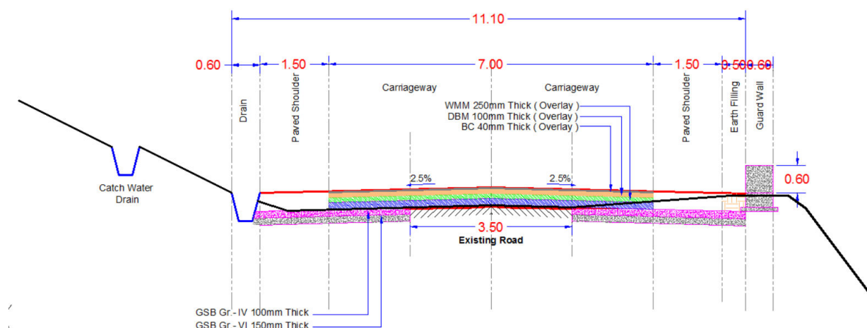
Figure B7: Typical Cross-section 5
