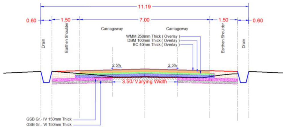
FigureB 4: Typical Cross-section 3
