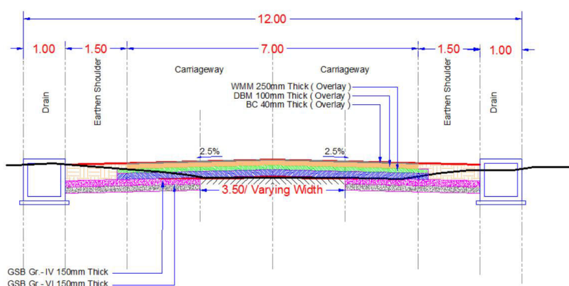
Figure B2: TYPICAL CROSS-SECTION 2
