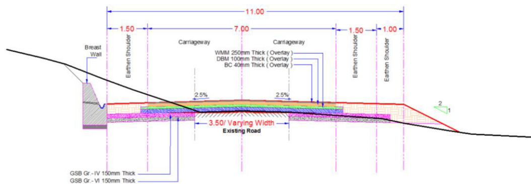
Figure B5: Typical Cross-section 3A
