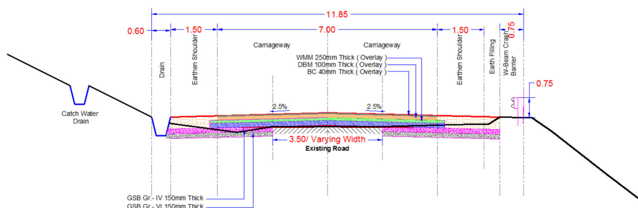
Figure B2: TYPICAL CROSS-SECTION 2
