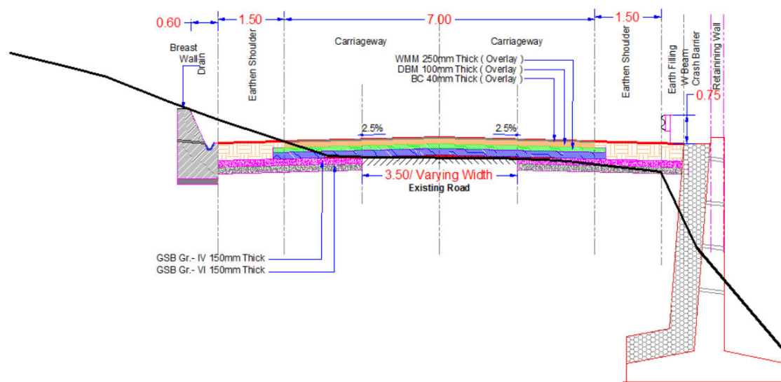
Figure B8: Typical Cross-section 6
